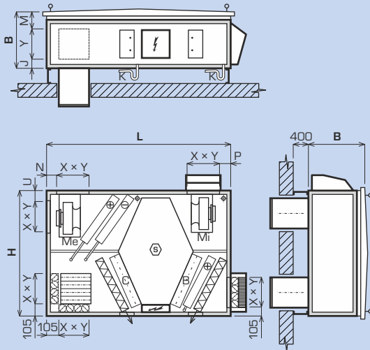
1500-6500 MultiEco-N configuration 4/16
