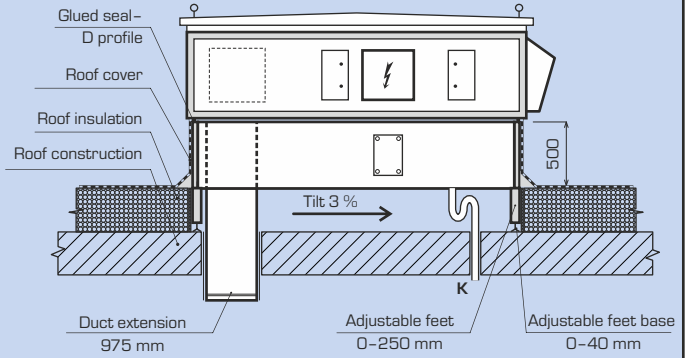
1500-6500 MultiEco-N
