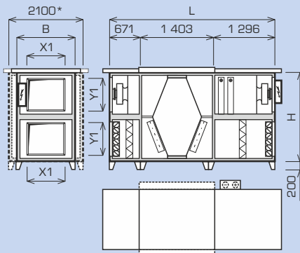
7500-9000 MultiEco-N configuration 10/0
