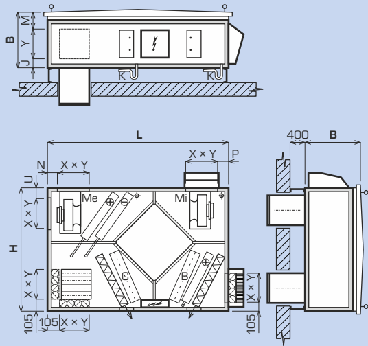
1400 - 10100 Basic-N configuration 4/16
