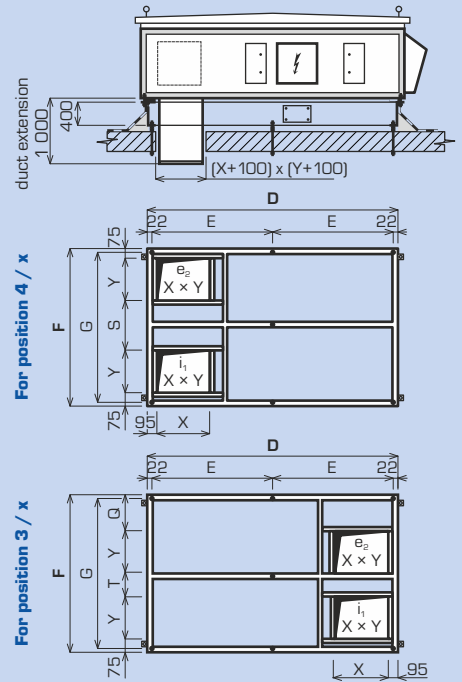
1400 - 10100 Basic-N
