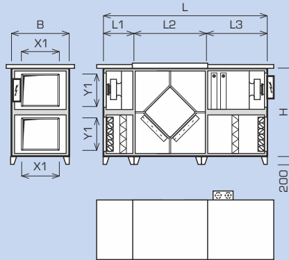
12'100 - 15100 Basic-N configuration 10/O and 11/O
