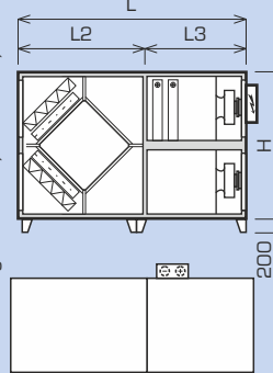
12'100 - 15100 Basic-N configuration 12/O and 13/O
