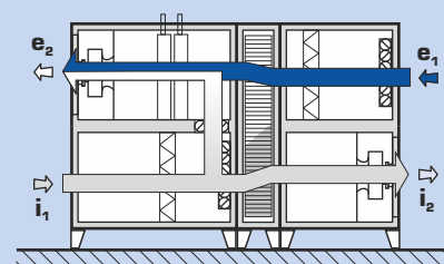
Combined mode (ventilation with circulation)
